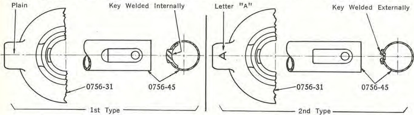
Cross Section of Lever Support and Shaft
