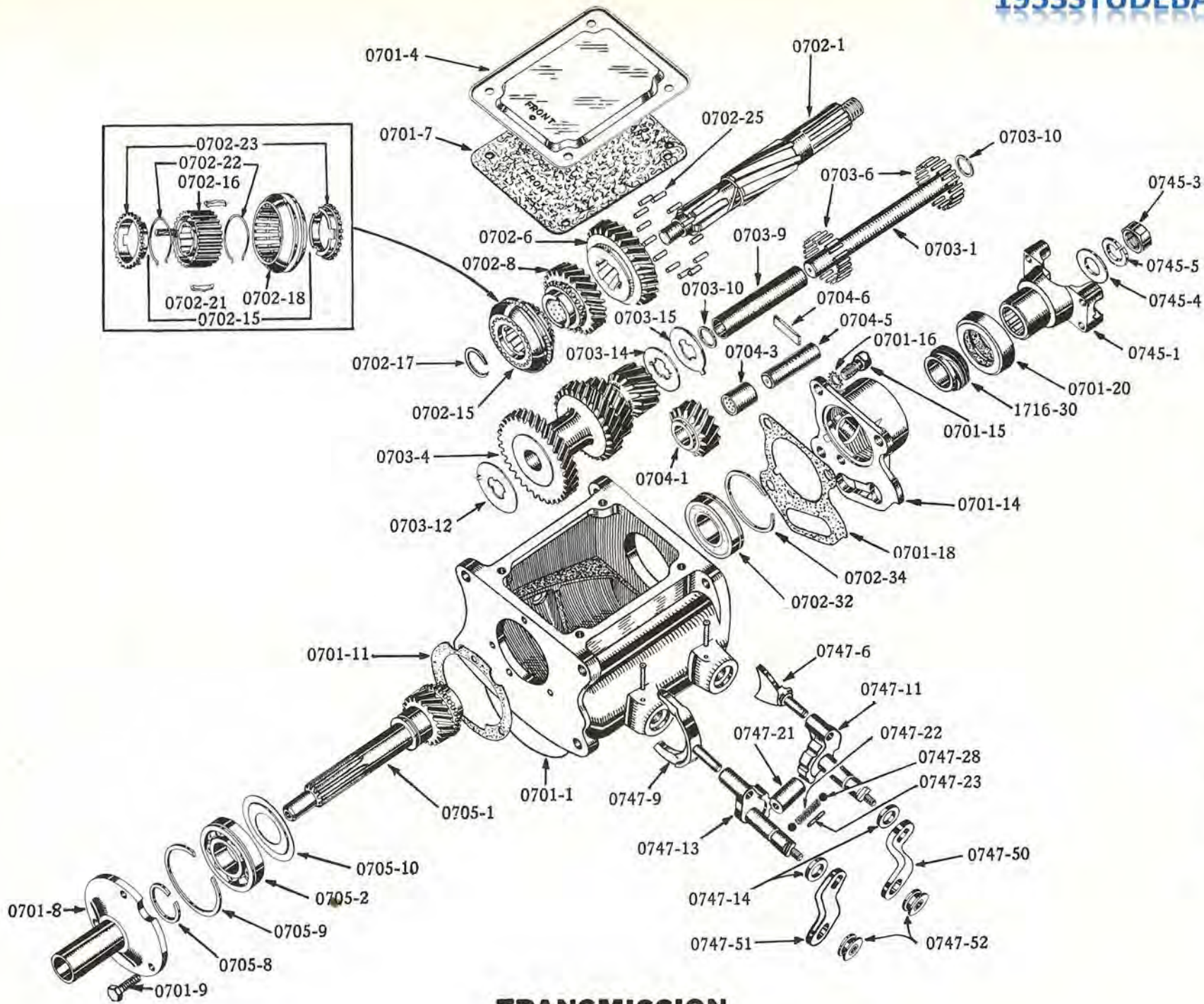
TRANSMISSION
