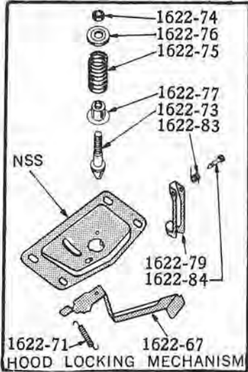
FENDERS, HOOD and MISC. SHEET METAL - Models 14G, 4H - C-K
