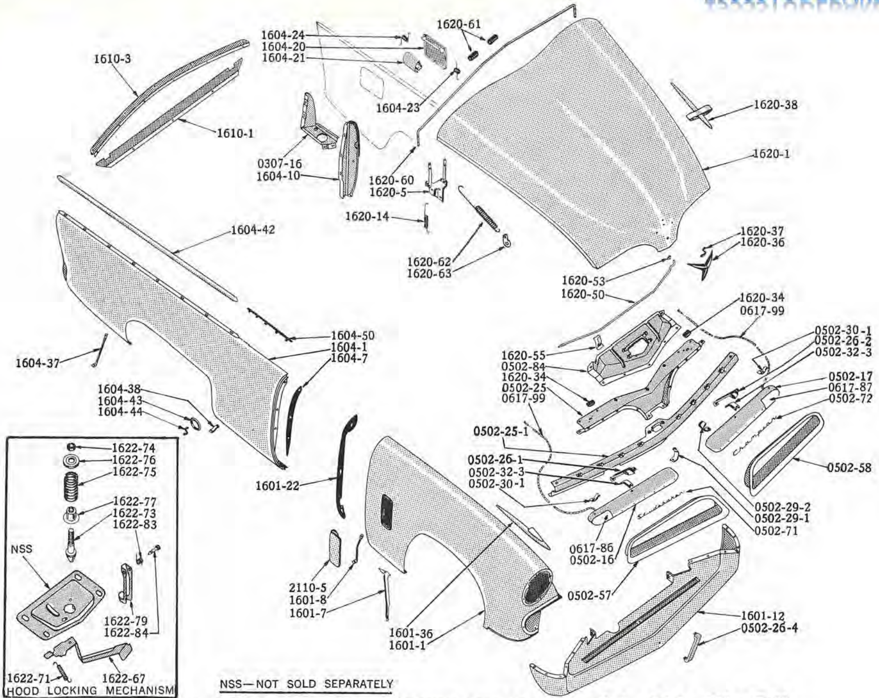
FENDERS, HOOD and MISC. SHEET METAL - Models 14G, 4H - C-K
