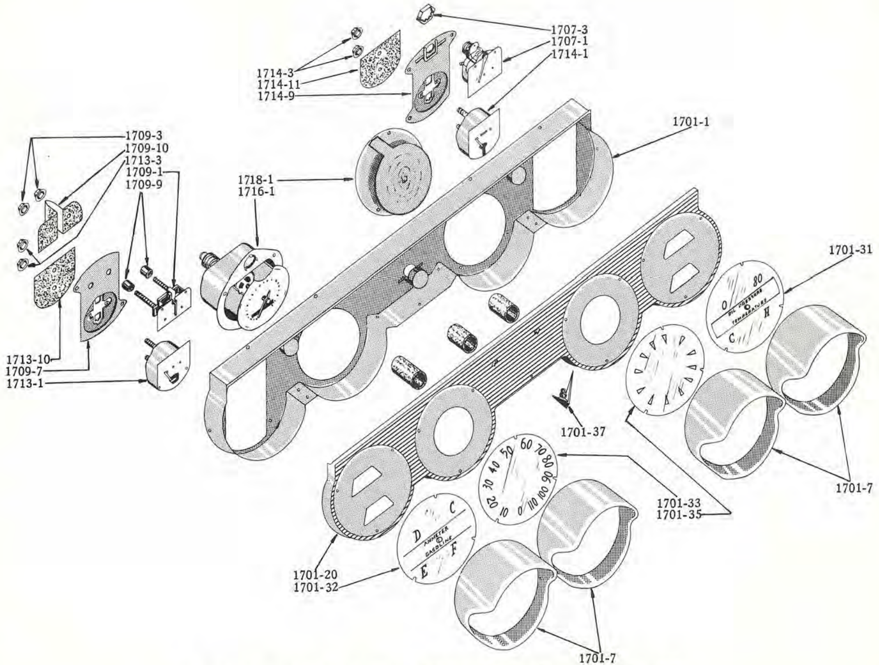
SPEEDOMETER and INSTRUMENTS - Model 4H
