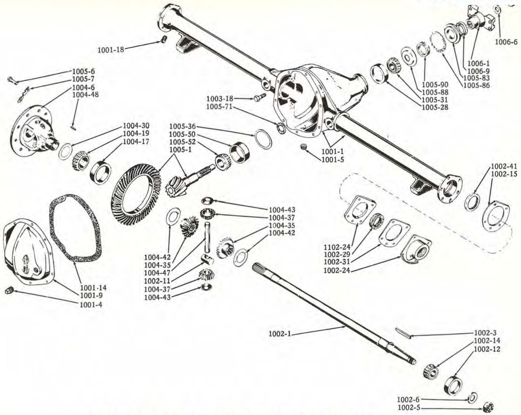
REAR AXLE and DIFFERENTIAL - Models H, 3H, 4H
